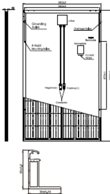
Dimensions of PV Module
